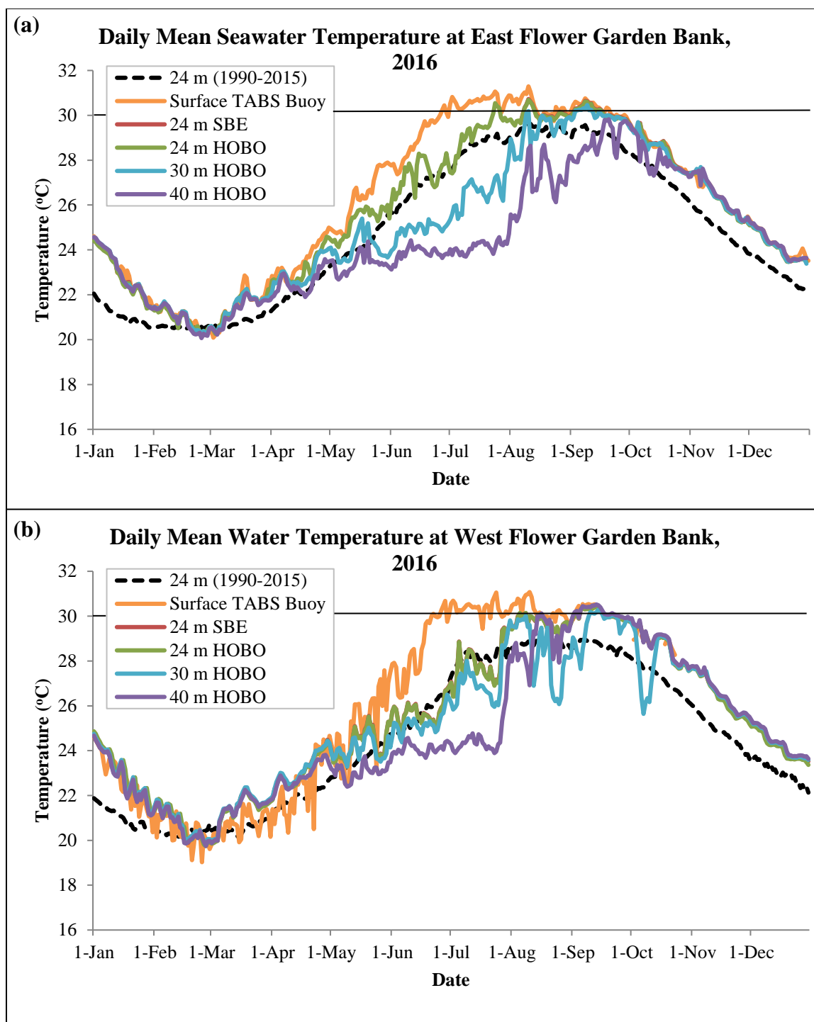
Figure 8.1. Daily mean water temperature (°C) at (a) EFGB and (b) WFGB from various depths in 2016 and 25-year daily mean temperature. Black represents 30°C bleaching threshold.
