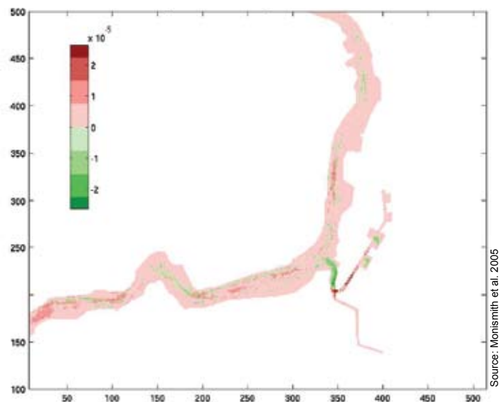
Figure 67. Erosion in the main channel of Elkhorn Slough as predicted by a computer model. Red areas show net erosion and green areas show net deposition over the course of the model run.
