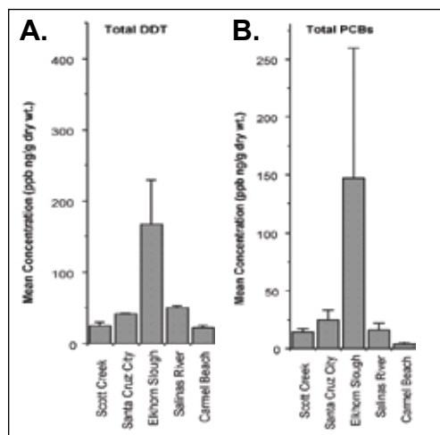
Figure 55. Mean dry weight concentrations (ng/g \pm 1 std. deviation) of total DDTs (DDD, DDE & DDT; Panel A) and total PCBs (Panel B) in tissues of sand crabs collected at beaches in August-September 2000.
