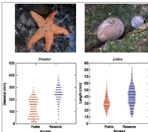
Figure 60. The size-frequency structure of the ochre star ( Pisaster ochraceus ) and the owl limpet ( Lottia gigantea ) are reduced in areas where the public has easy access to the rocky shore (red bars) compared to areas where public access is difficult or prohibited (blue bars). The width of the bars indicates the number of animals of a given size.
