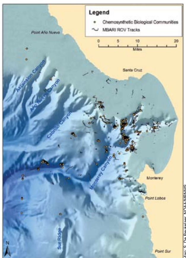
Figure 36. The location where cold seeps (orange circles) have been observed in the Monterey Bay region. Black lines show the locations where the Monterey Bay Aquarium Research Institute (MBARI) conducted remotely operated vehicle (ROV) surveys from April 1989 to June 2002.
