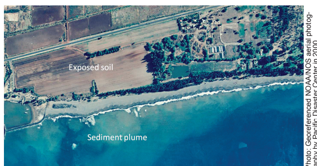
Figure 13. A sediment plume in this aerial photograph off the coast of Kaua'i. The sediment was transported by runoff from fields where soil is exposed.
