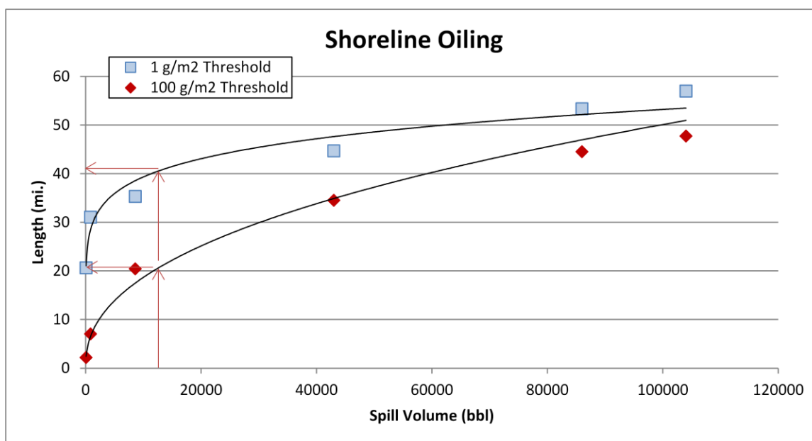
Figure 2-4: Regression curve for estimating the amount of shoreline oiling at different thresholds as a function of spill volume for the Virginia , based on the model results for the R.W. Gallagher . The arrows indicate where the WCD for the Virginia falls on the curve and how the length of shoreline impact can be determined for any spill volume.
