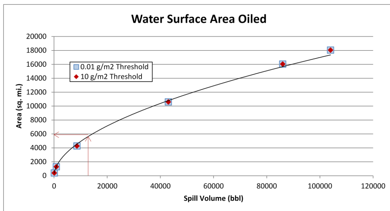
Figure 2-3: Regression curve for estimating the amount of water surface oiling as a function of spill volume for the Virginia , showing both the ecological threshold of 10 g/m 2 and socio-economic threshold of 0.01 g/m 2 , based on the model results for the R.W. Gallagher . The arrows indicate where the WCD for the Virginia falls on the curve and how the area of water surface impact can be determined for any spill volume. The curves for each threshold are so similar that they plot on top of each other.
