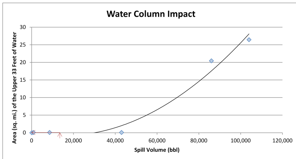
Figure 2-2: Regression curve for estimating the area of water column at or above 1 ppb aromatics impacted as a function of spill volume for the Virginia . This regression curve was generated for the R.W. Gallagher , which has the same oil type and similar volume of potential releases as the Virginia . The arrows indicate where the WCD for the Virginia falls on the curve and how the area of water column impact can be determined for any spill volume.
