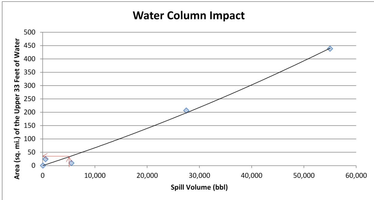
Figure 2-2: Regression curve for estimating the area of water column at or above 1 ppb aromatics impacted as a function of spill volume for the Vainqueur . This regression curve was generated for the Gulfoil , which has the same oil type and similar volume of potential releases as the Vainqueur . The arrows indicate where the WCD for the Vainqueur falls on the curve and how the area of water column impact can be determined for any spill volume.
