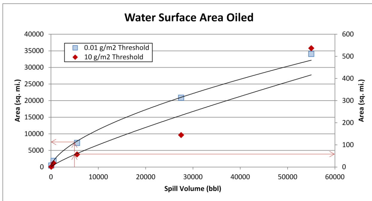
Figure 2-3: Regression curve for estimating the amount of water surface oiling as a function of spill volume for the Vainqueur , showing both the ecological threshold of 10 g/m 2 (use the scale on the right side of the plot) and socio-economic threshold of 0.01 g/m 2 (use the scale on the left side of the plot), based on the model results for the Gulfoil . The arrows indicate where the WCD for the Vainqueur falls on the curve and how the area of water surface impact can be determined for any spill volume.
