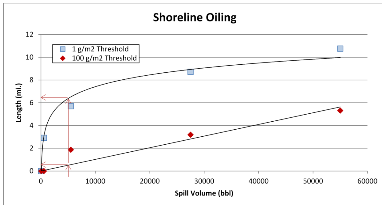
Figure 2-4: Regression curve for estimating the amount of shoreline oiling at different thresholds as a function of spill volume for the Vainqueur , based on the model results for the Gulfoil . The arrows indicate where the WCD for the Vainqueur falls on the curve and how the length of shoreline impact can be determined for any spill volume.
