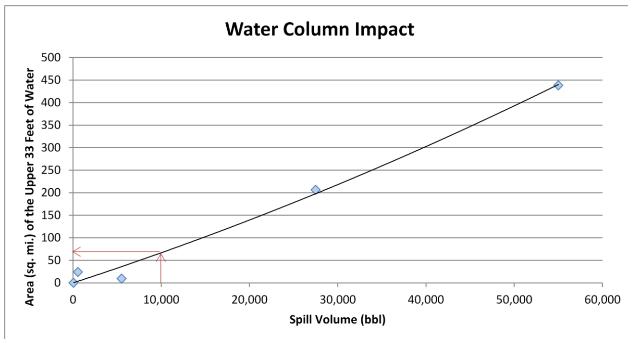
Figure 2-2: Regression curve for estimating the area of water column at or above 1 ppb aromatics impacted as a function of spill volume for the Sheherazade . This regression curve was generated for the Gulfoil , which has the same oil type and similar volume of potential releases as the Sheherazade . The arrows indicate where the WCD for the Sheherazade falls on the curve and how the area of water column impact can be determined for any spill volume.
