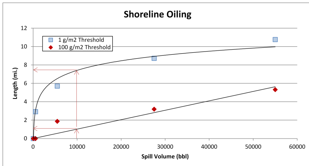
Figure 2-4: Regression curve for estimating the amount of shoreline oiling at different thresholds as a function of spill volume for the Sheherazade , based on the model results for the Gulfoil . The arrows indicate where the WCD for the Sheherazade falls on the curve and how the length of shoreline impact can be determined for any spill volume.
