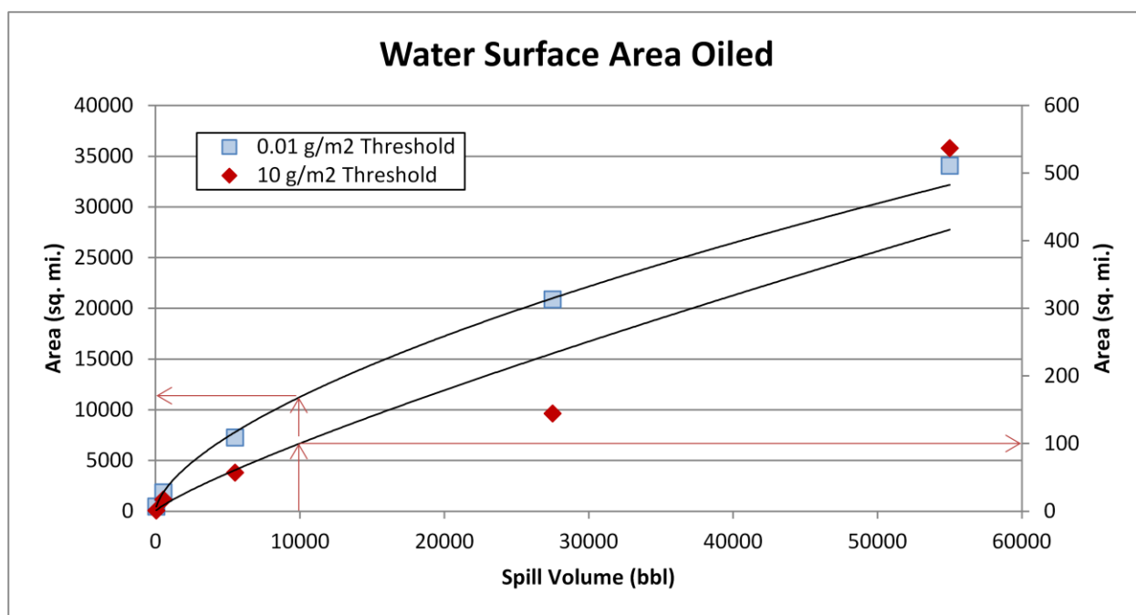
Figure 2-3: Regression curve for estimating the amount of water surface oiling as a function of spill volume for the Sheherazade , showing both the ecological threshold of 10 g/m 2 (use the scale on the right side of the plot) and socio-economic threshold of 0.01 g/m 2 (use the scale on the left side of the plot), based on the model results for the Gulfoil . The arrows indicate where the WCD for the Sheherazade falls on the curve and how the area of water surface impact can be determined for any spill volume.
