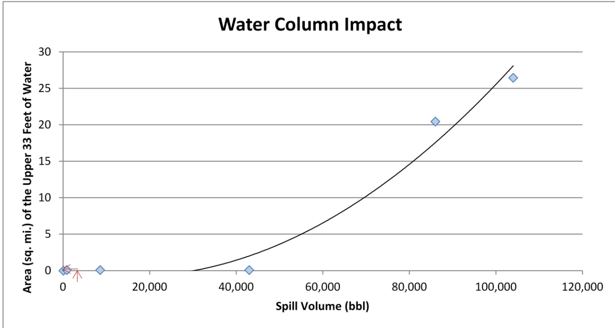
Figure 2-2: Regression curve for estimating the area of water column at or above 1 ppb aromatics impacted as a function of spill volume for the Rawleigh Warner . This regression curve was generated for the R.W. Gallagher , which has the same oil type as the Rawleigh Warner . The arrows indicate where the WCD for the Rawleigh Warner falls on the curve and how the area of water column impact can be determined for any spill volume.
