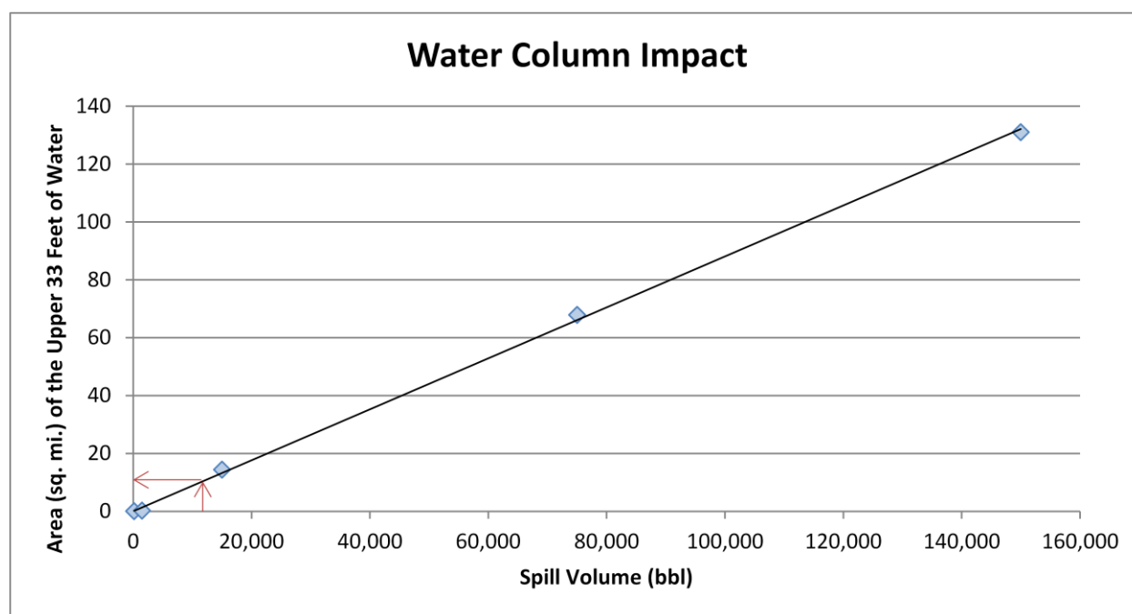
Figure 2-2: Regression curve for estimating the area of water column at or above 1 ppb aromatics impacted as a function of spill volume for the Paestum . This regression curve was generated for the William Rockefeller , which has the same oil type and similar volume of potential releases as the Paestum . The arrows indicate where the WCD for the Paestum falls on the curve and how the area of water column impact can be determined for any spill volume.
