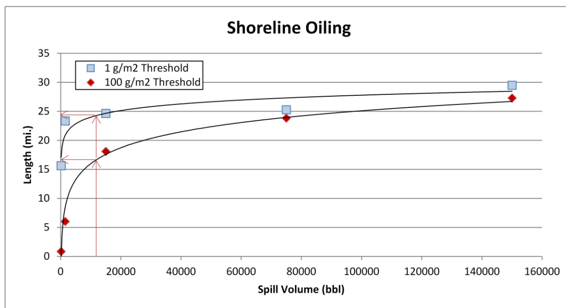
Figure 2-4: Regression curve for estimating the amount of shoreline oiling at different thresholds as a function of spill volume for the Paestum , based on the model results for the William Rockefeller . The arrows indicate where the WCD for the Paestum falls on the curve and how the length of shoreline impact can be determined for any spill volume.
