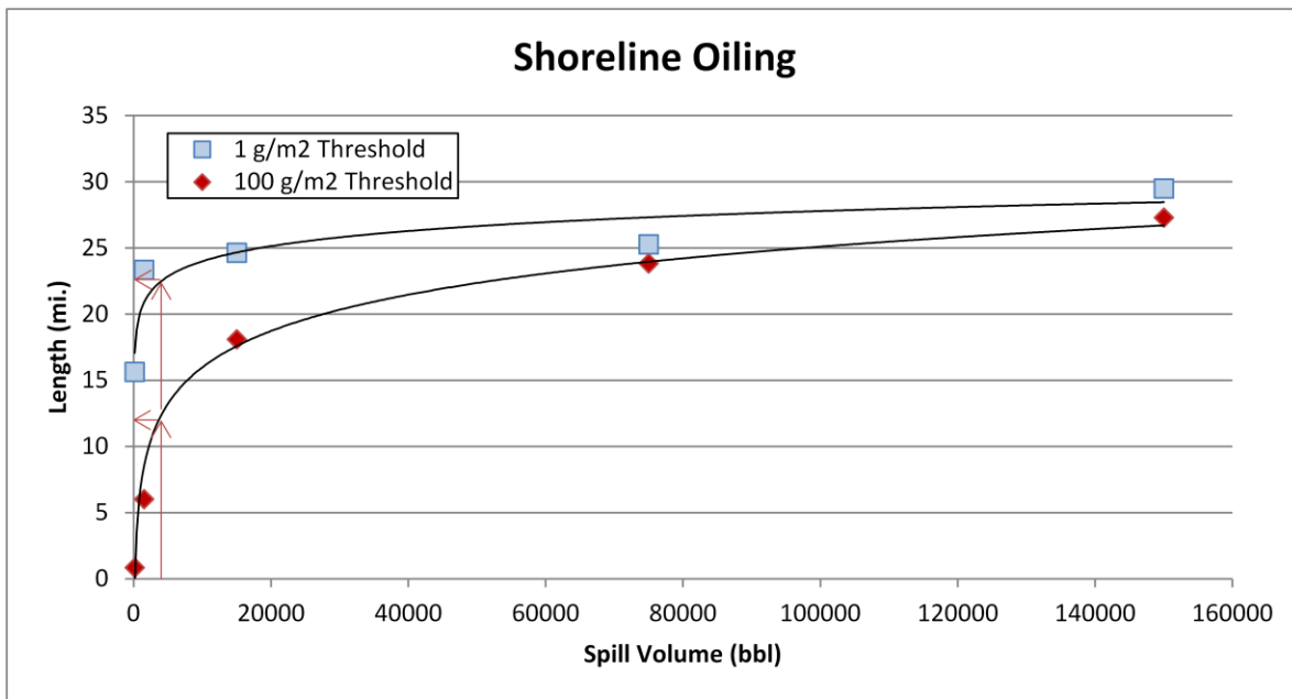
Figure 2-4: Regression curve for estimating the amount of shoreline oiling at different thresholds as a function of spill volume for the Norlavore , based on the model results for the William Rockefeller . The arrows indicate where the WCD for the Norlavore falls on the curve and how the length of shoreline impact can be determined for any spill volume.
