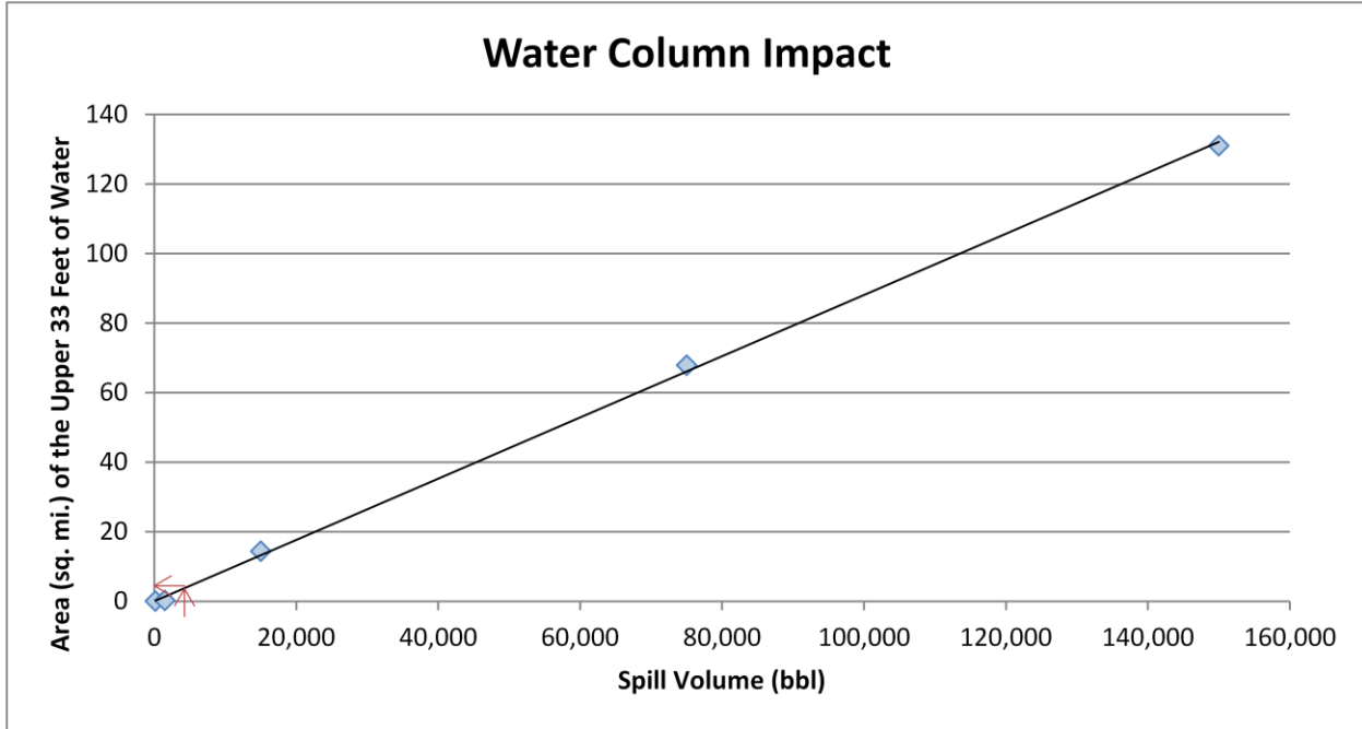
Figure 2-2: Regression curve for estimating the area of water column at or above 1 ppb aromatics impacted as a function of spill volume for the Norlavore . This regression curve was generated for the William Rockefeller , which has the same oil type and similar volume of potential releases as the Norlavore . The arrows indicate where the WCD for the Norlavore falls on the curve and how the area of water column impact can be determined for any spill volume.
