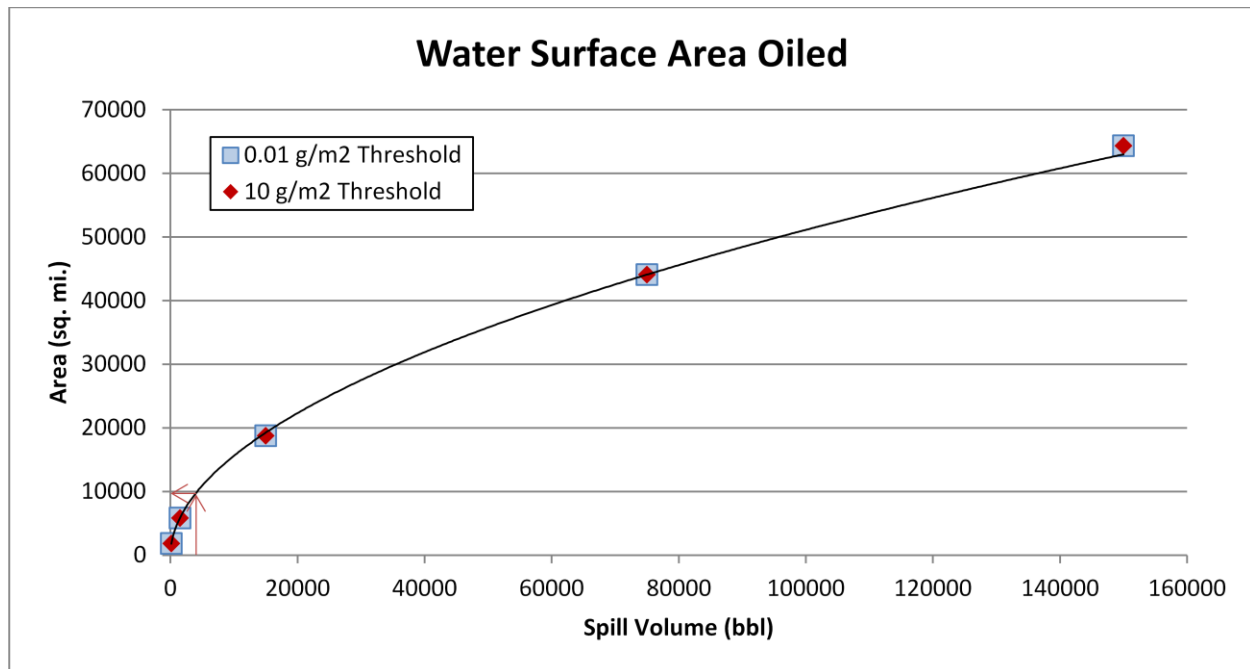
Figure 2-3: Regression curve for estimating the amount of water surface oiling as a function of spill volume for the Norlavore , showing both the ecological threshold of 10 g/m 2 and socio-economic threshold of 0.01 g/m 2 , based on the model results for the William Rockefeller . The arrows indicate where the WCD for the Norlavore falls on the curve and how the area of water surface impact can be determined for any spill volume. The curves for each threshold are so similar that they plot on top of each other.
