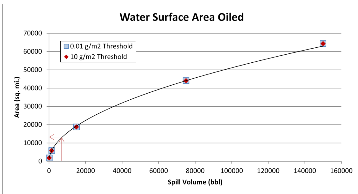
Figure 2-3: Regression curve for estimating the amount of water surface oiling as a function of spill volume for the Ljubica Matkovic , showing both the ecological threshold of 10 g/m 2 and socio-economic threshold of 0.01 g/m 2 , based on the model results for the William Rockefeller . The arrows indicate where the WCD for the Ljubica Matkovic falls on the curve and how the area of water surface impact can be determined for any spill volume. The curves for each threshold are so similar that they plot on top of each other.
