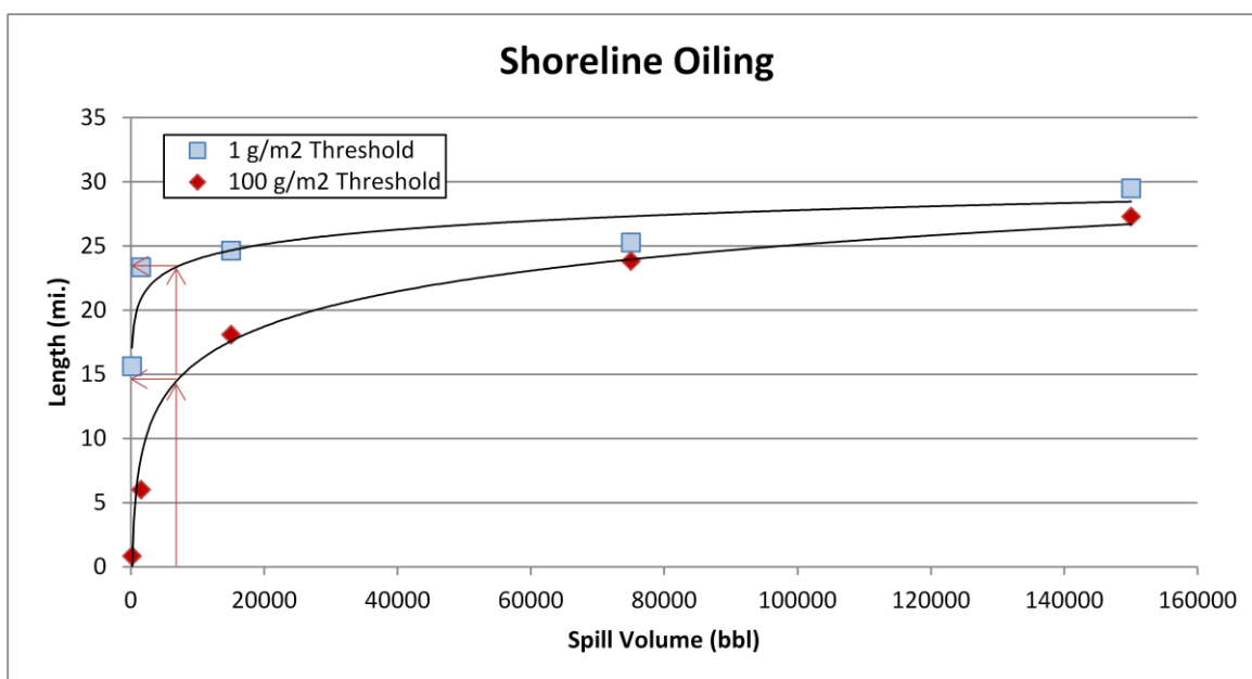
Figure 2-4: Regression curve for estimating the amount of shoreline oiling at different thresholds as a function of spill volume for the Ljubica Matkovic , based on the model results for the William Rockefeller . The arrows indicate where the WCD for the Ljubica Matkovic falls on the curve and how the length of shoreline impact can be determined for any spill volume.
