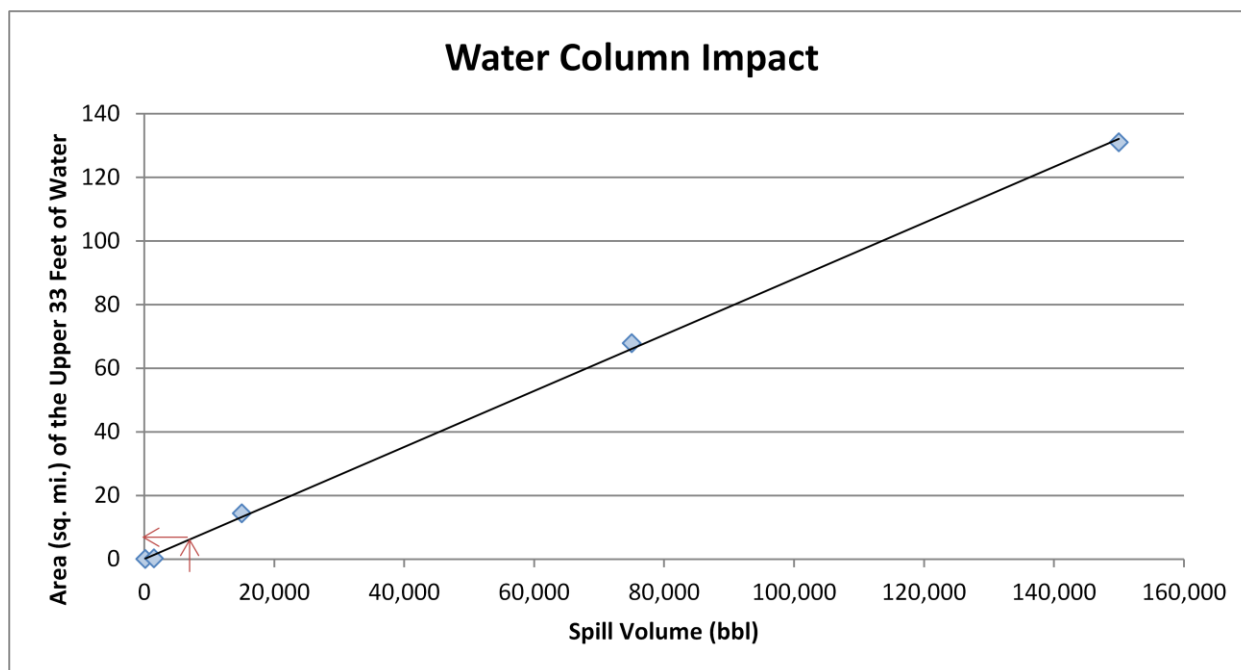
Figure 2-2: Regression curve for estimating the area of water column at or above 1 ppb aromatics impacted as a function of spill volume for the Ljubica Matkovic . This regression curve was generated for the William Rockefeller , which has the same oil type and similar volume of potential releases as the Ljubica Matkovic . The arrows indicate where the WCD for the Ljubica Matkovic falls on the curve and how the area of water column impact can be determined for any spill volume.
