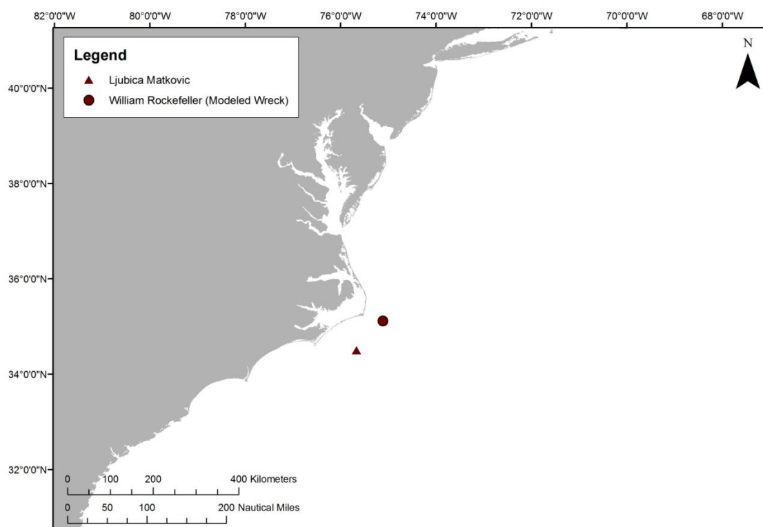
Figure 2-1: Location of the Ljubica Matkovic (red triangle), the wreck discussed in this package, and the William Rockefeller (red circle) which was the wreck that was actually modeled in the computer modeling simulations. The results for the William Rockefeller are used to estimate the impacts of releases from the Ljubica Matkovic , as discussed in the text.
