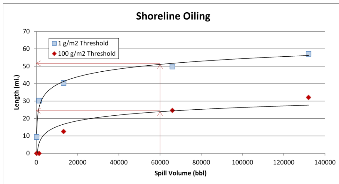
Figure 2-4: Regression curve for estimating the amount of shoreline oiling at different thresholds as a function of spill volume for the Doris Kellogg , based on the model results for the Esso Gettysburg . The arrows indicate where the WCD for the Doris Kellogg falls on the curve and how the length of shoreline impact can be determined for any spill volume.
