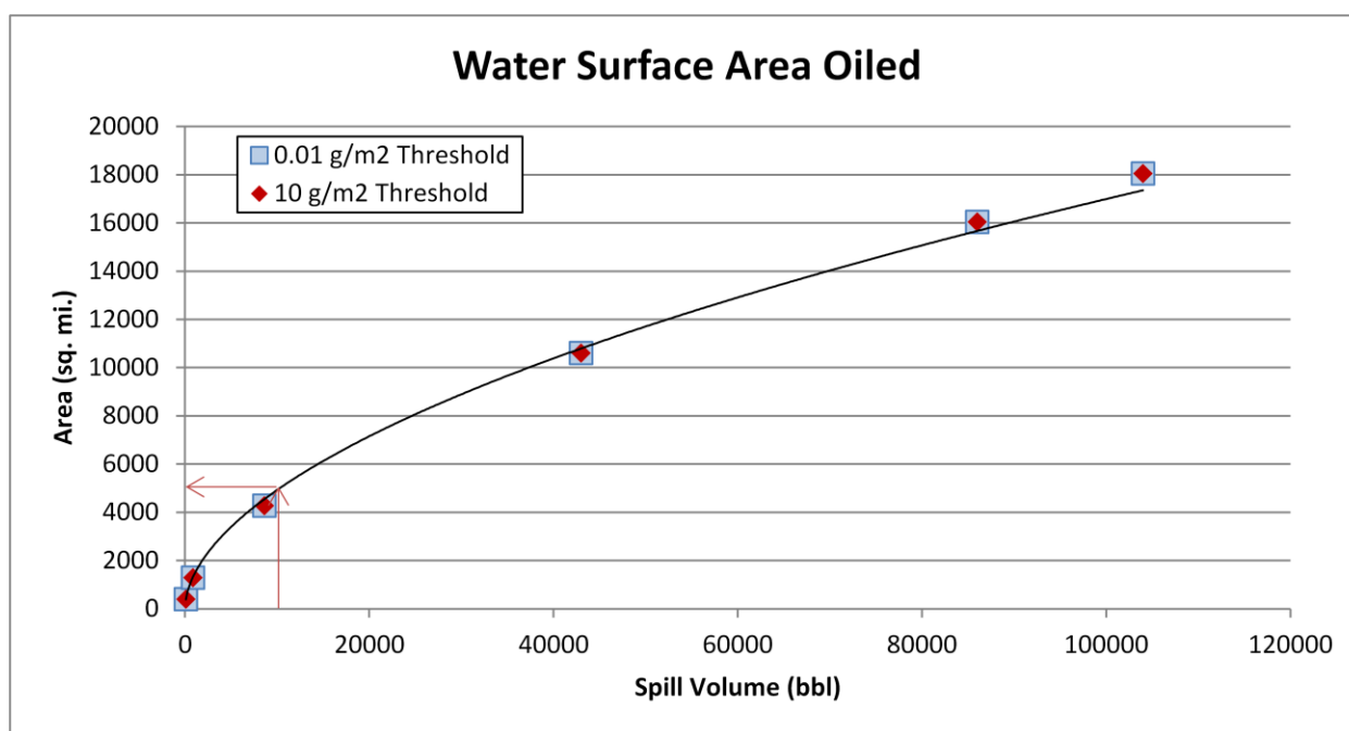
Figure 2-3: Regression curve for estimating the amount of water surface oiling as a function of spill volume for the Alcoa Puritan , showing both the ecological threshold of 10 g/m 2 and socio-economic threshold of 0.01 g/m 2 , based on the model results for the R.W. Gallagher . The arrows indicate where the WCD for the Alcoa Puritan falls on the curve and how the area of water surface impact can be determined for any spill volume. The curves for each threshold are so similar that they plot on top of each other.
