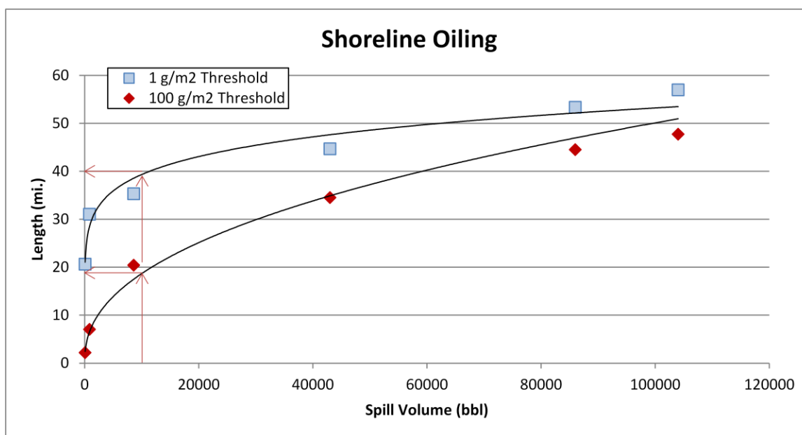
Figure 2-4: Regression curve for estimating the amount of shoreline oiling at different thresholds as a function of spill volume for the Alcoa Puritan , based on the model results for the R.W. Gallagher . The arrows indicate where the WCD for the Alcoa Puritan falls on the curve and how the length of shoreline impact can be determined for any spill volume.
