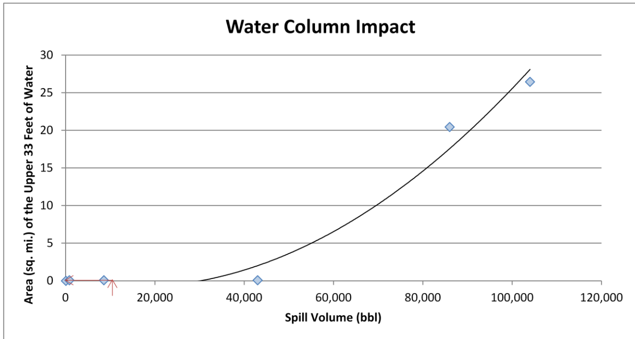
Figure 2-2: Regression curve for estimating the area of water column at or above 1 ppb aromatics impacted as a function of spill volume for the Alcoa Puritan . This regression curve was generated for the R.W. Gallagher , which has the same oil type and similar volume of potential releases as the Alcoa Puritan . The arrows indicate where the WCD for the Alcoa Puritan falls on the curve and how the area of water column impact can be determined for any spill volume.
