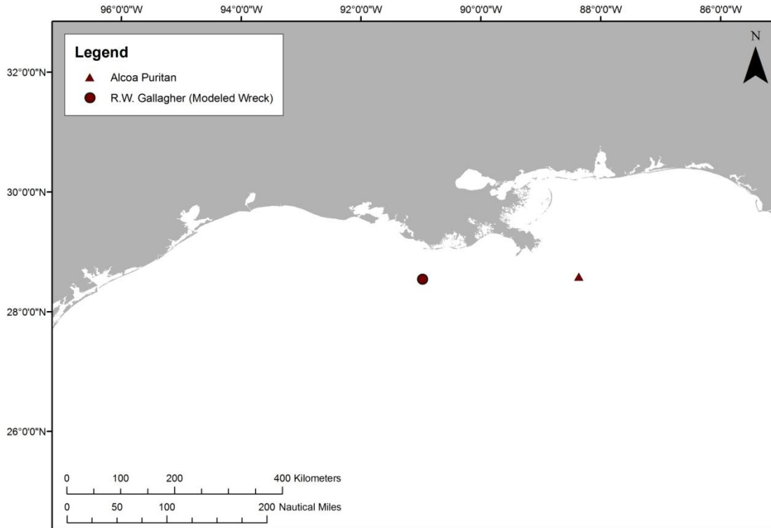
Figure 2-1: Location of the Alcoa Puritan (red triangle), the wreck discussed in this package, and the R.W. Gallagher (red circle) which was the wreck that was actually modeled in the computer modeling simulations. The results for the R.W. Gallagher are used to estimate the impacts of releases from the Alcoa Puritan , as discussed in the text.
